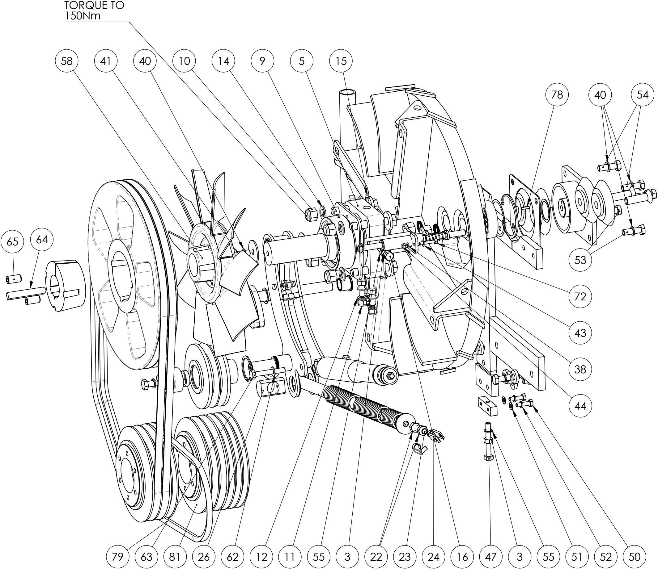
301020113 ARB200 FLYWHEEL DRIVE DETAIL
