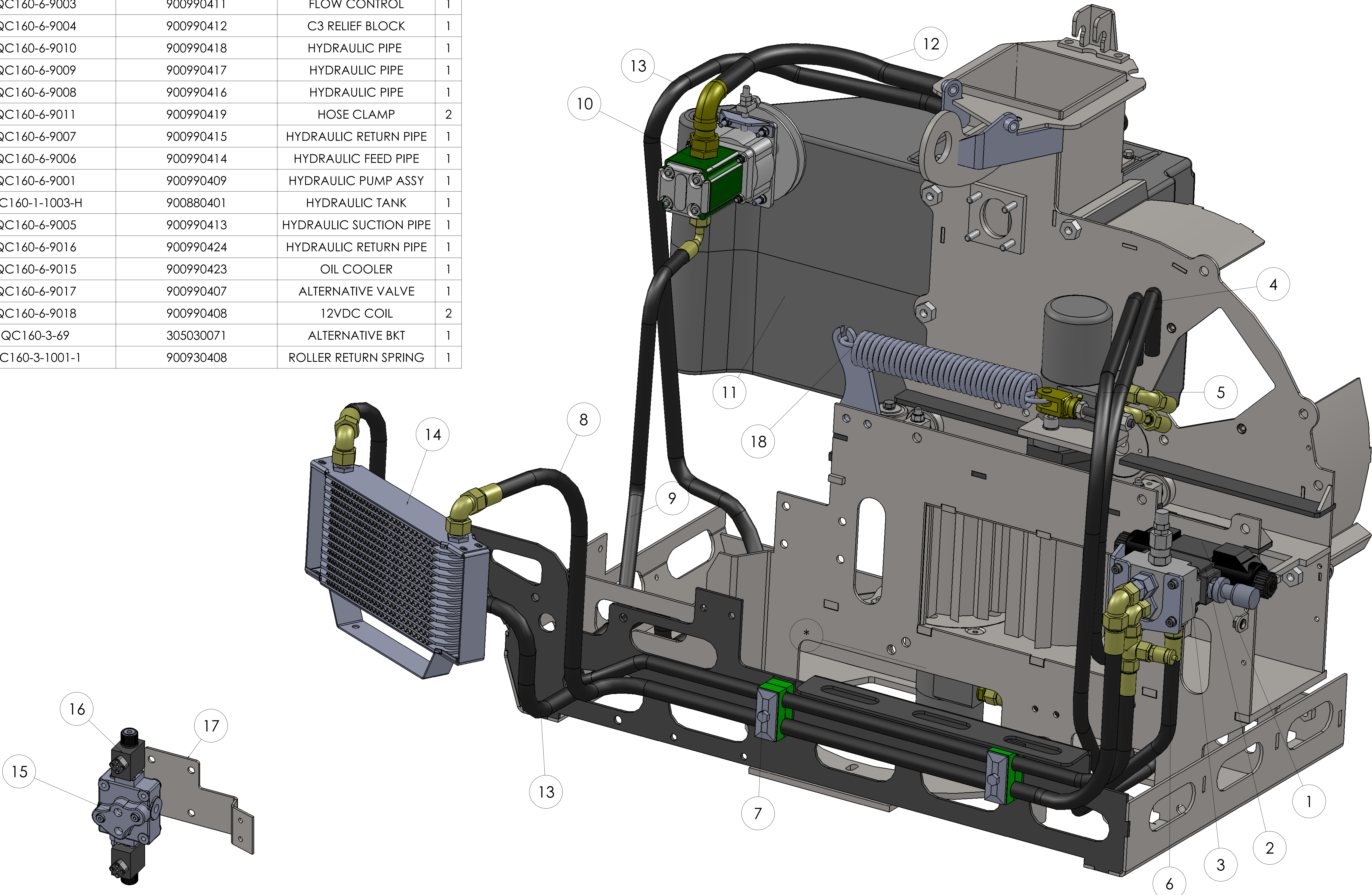
HYDRAULIC LAYOUT WITH OIL COOLER
